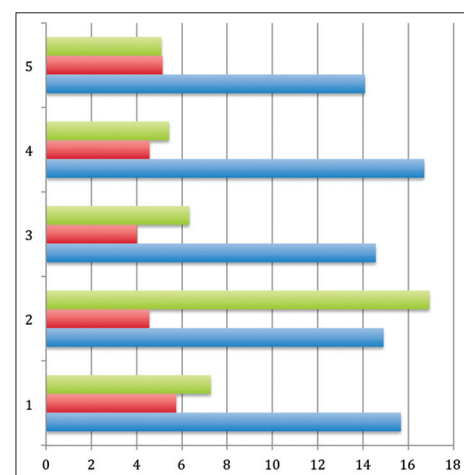
Figure 2: Delta E for specimens used in coffee, Blue column represent DE of Filtek 350XT, the red column represent DE of Ceram X due, while green column represent DE of Venus Diamond
