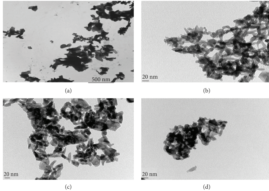
FIGURE 2: TEM micrographs for \text{Zn}_{1-x}\text{Sm}_x\text{O} with (a) x = 0.00 , (b) x = 0.01 , (c) x = 0.06 , and (d) x = 0.10 .
