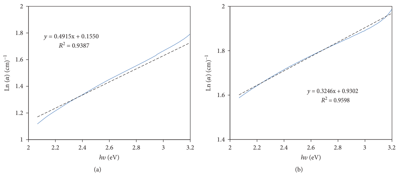
FIGURE 6: \ln(\alpha) versus photon energy ( h\nu ) is shown in the inset for (a) x = 0.00 and (b) x = 0.08 .
