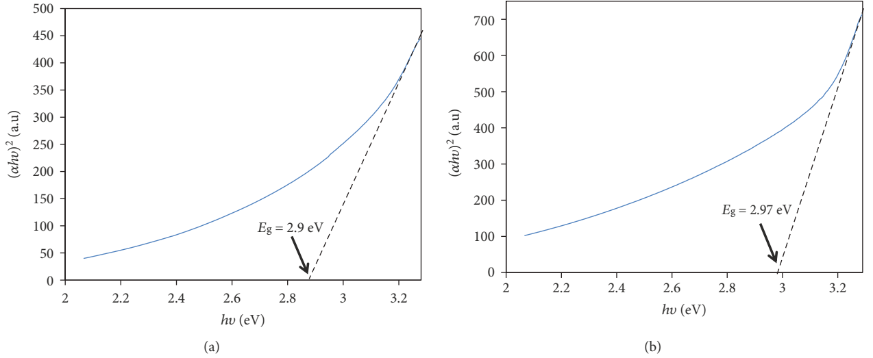
FIGURE 5: (\alpha h\nu)^2 versus photon energy ( h\nu ) of \text{Zn}_{1-x}\text{Sm}_x\text{O} for (a) x = 0.00 and (b) x = 0.08 .
