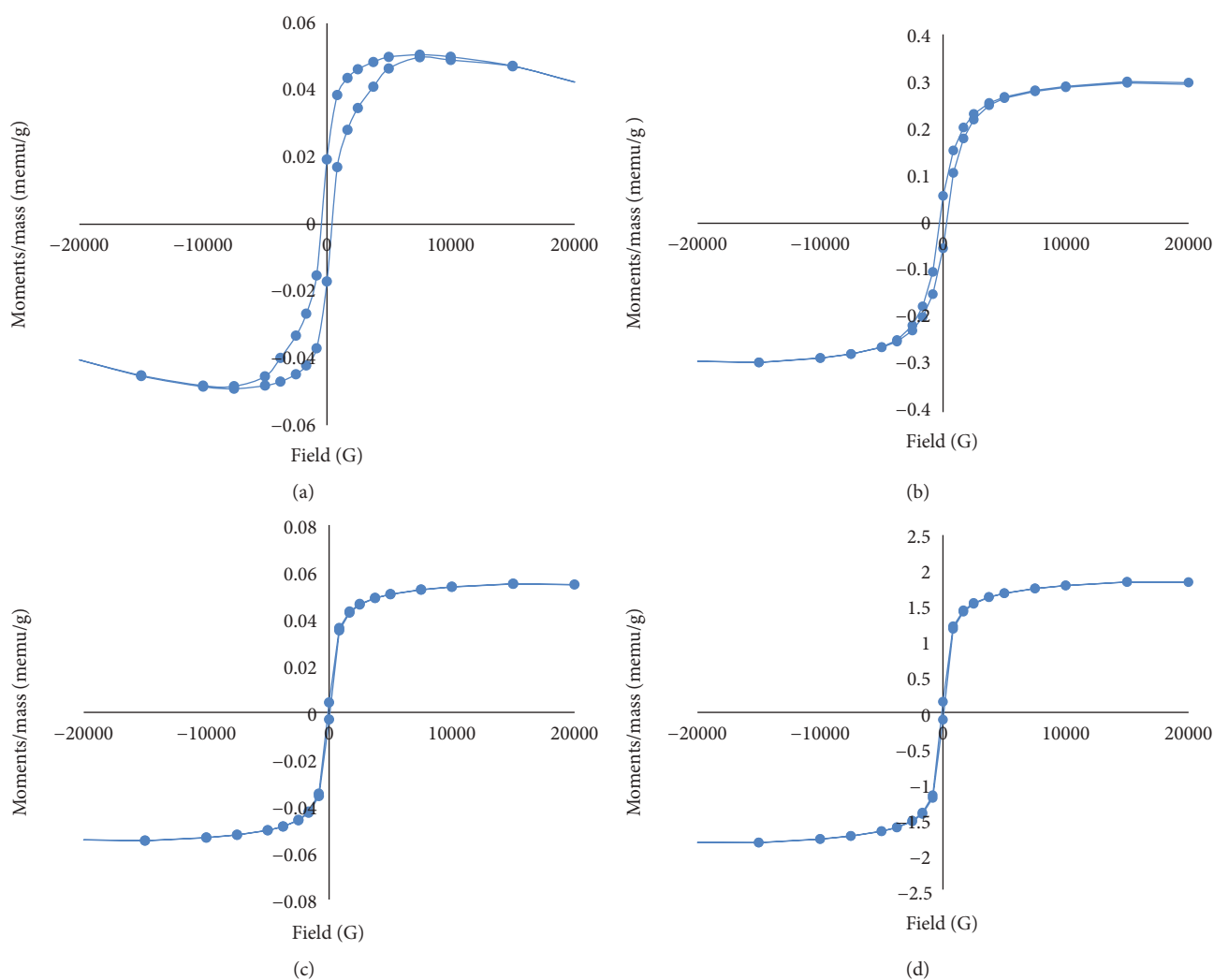
FIGURE 7: (M-H) hysteresis loop of \text{Zn}_{1-x}\text{Sm}_x\text{O} nanoparticles for (a) x = 0.00 , (b) x = 0.01 , (c) x = 0.08 , and (d) x = 0.10 .
