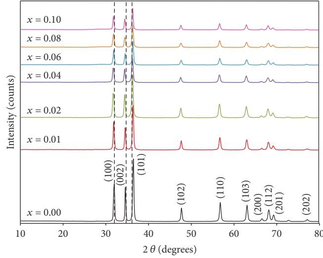
FIGURE 1: XRD patterns of \text{Zn}_{1-x}\text{Sm}_x\text{O} for 0.01 \leq x \leq 0.10 .
