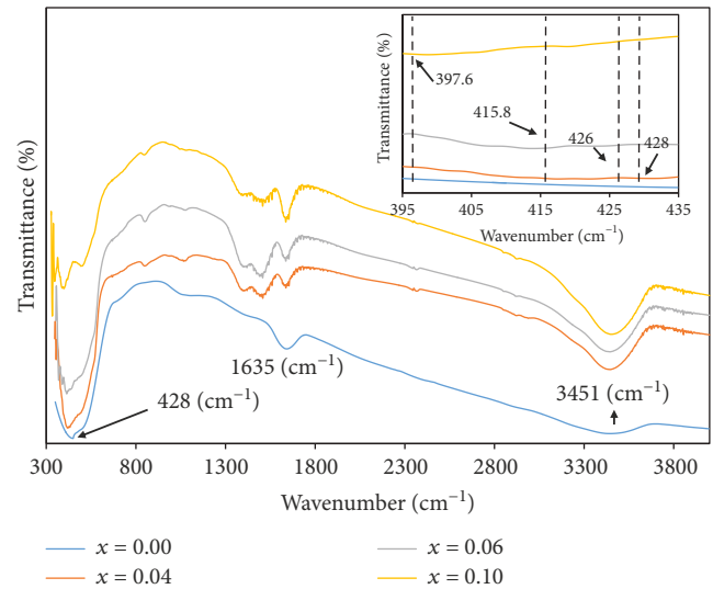
FIGURE 3: FTIR spectra of \text{Zn}_{1-x}\text{Sm}_x\text{O} nanoparticles with x = 0.00, x = 0.04, x = 0.06 , and x = 0.10 . The inset shows the absorption peaks of \text{Zn}_{1-x}\text{Sm}_x\text{O} with x = 0.00, x = 0.04, x = 0.06 , and x = 0.10 at Zn-O stretching vibration.
