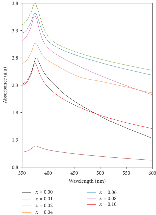
FIGURE 4: The UV-visible spectroscopy of \text{Zn}_{1-x}\text{Sm}_x\text{O} for 0.01 \leq x \leq 0.10 .
